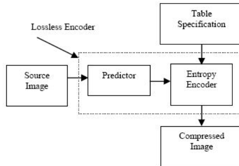
Fig :Block Diagram for Lossless Compression
